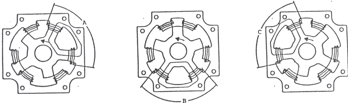
FIG. 7A 6/5 3 PHASE
