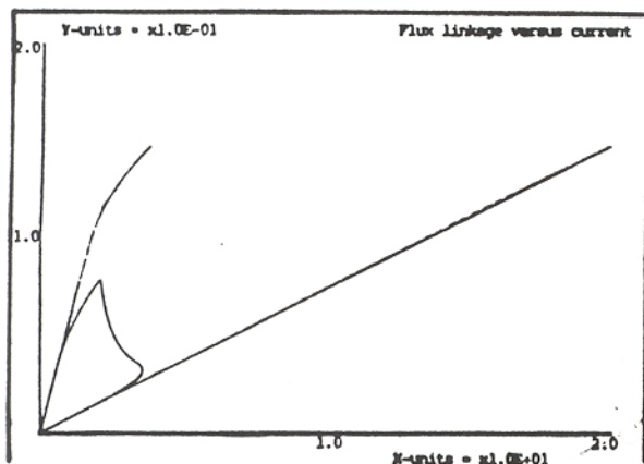
FIG. 2- PCSRD Performance Modler results. (University of Glasgow)
