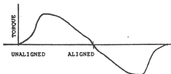
TORQUE VS ROTOR ANGLE TYPICAL VR STEPPING MOTOR
