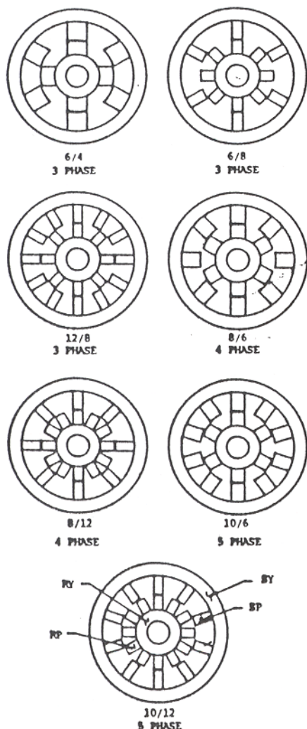
VR BRUSHLESS POLE & PHASE ARRANGEMENT
